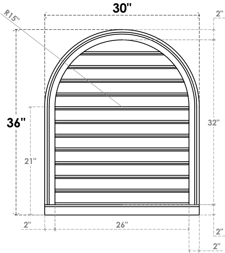
FRONT
